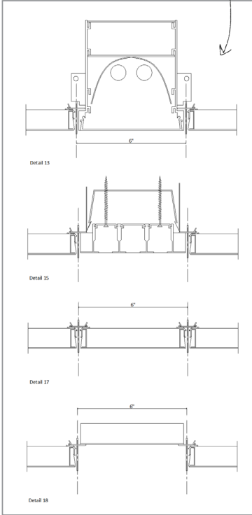
INTEGRATED LIGHTS/DIFFUSERS
